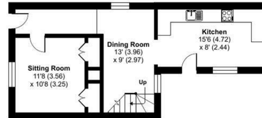
MOUNT VIEW COTTAGE - GROUND FLOOR
